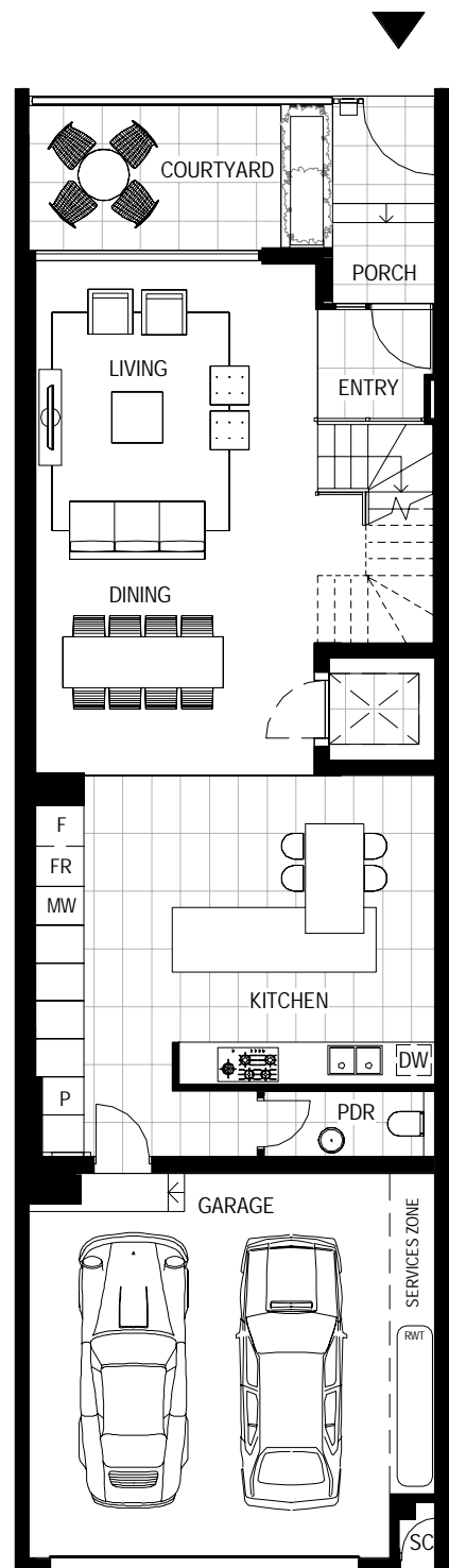
GROUND FLOOR
